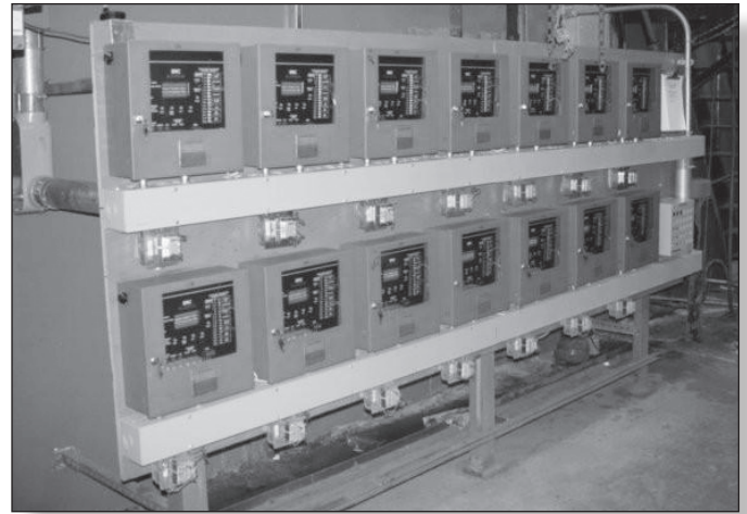
Multiple SRC Platinum Steam Reset Controls, all tied into a Heat-Timer ICMS Internet Communications Management System, keep fuel cost down while drastically reducing maintenance legwork at Big Six.
